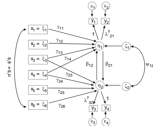
Figure 14. Latent-variable model for the peer-influences data.
